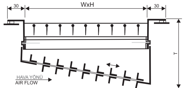
DAMPERLİ / WITH DAMPER
