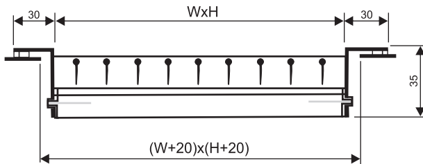
DAMPERSİZ / WITHOUT DAMPER
