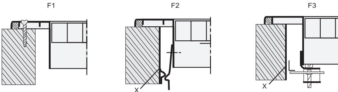
X=Kör kasa (Müşteriye aittir) / Mounting frame (Not by EGEVENT)
